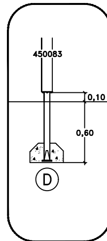
Cast In Place CC
